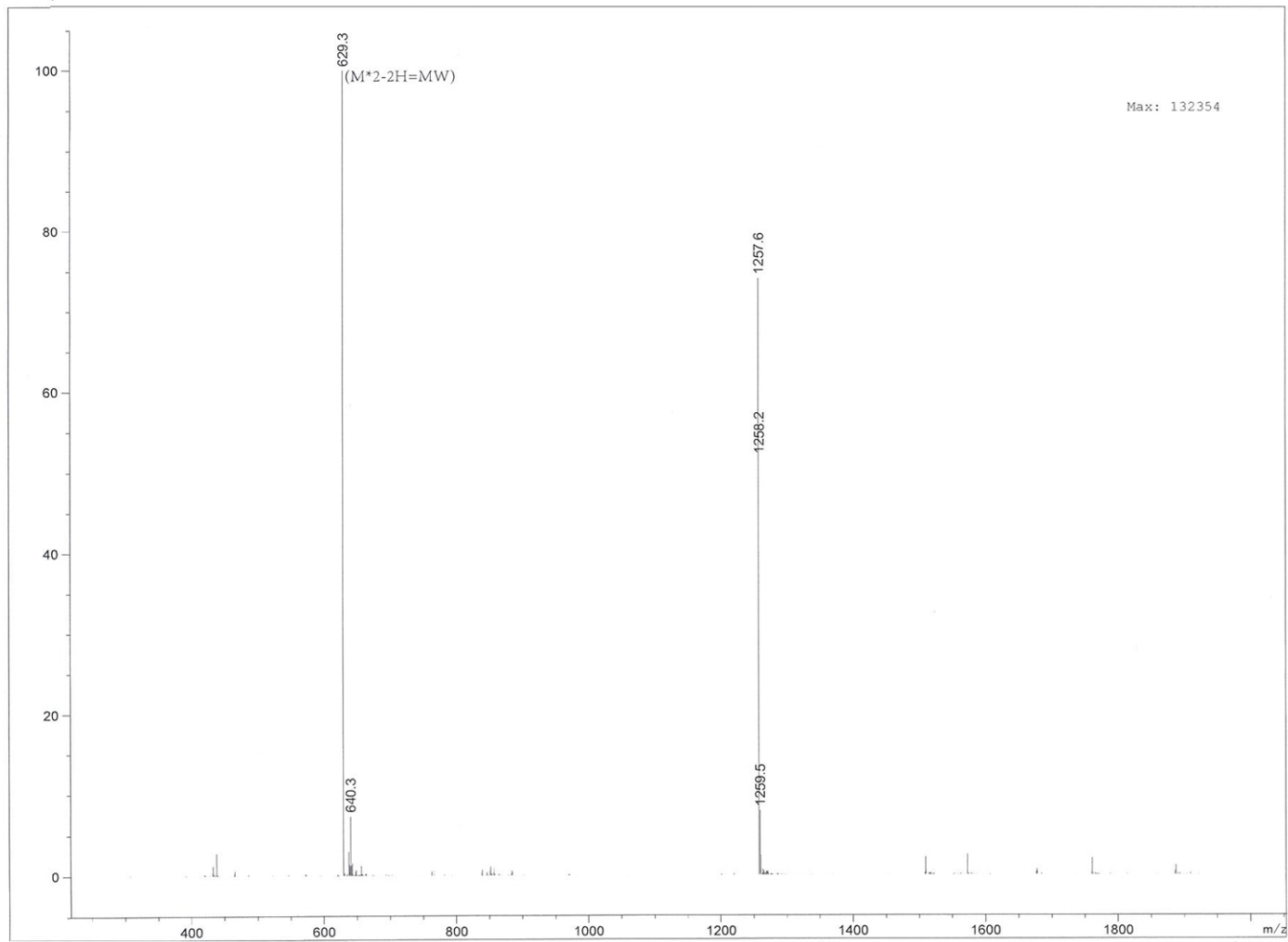
MS Spectrum
